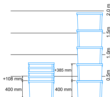
Ref. 980_ _ (ext.) 600x400x400mm (int.) 490x332x395mm 70L
