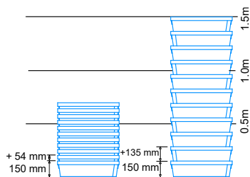
Ref. 990_ _ (ext.) 600x400x150mm (int.) 490x332x145mm 25L
