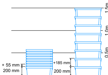
Ref. 970_ _ (ext.) 600x400x200mm (int.) 490x332x195mm 35L
