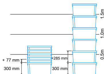
Ref. 975_ _ (ext.) 600x400x300mm (int.) 490x332x295mm 50L
