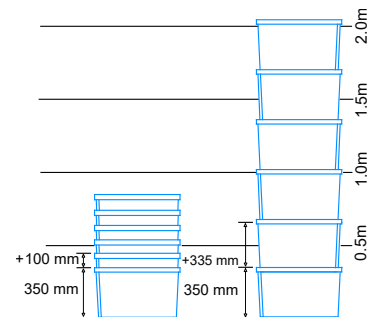
Ref. 235_ _ (ext.) 600x400x350mm (int.) 490x340x347mm 66L
