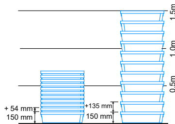
Ref. 990__ (ext.) 600x400x150mm (int.) 490x332x145mm
