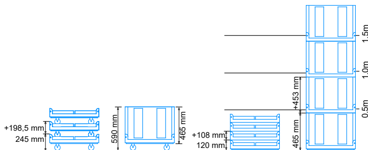
Ref. 962_ _ (ext.) 800x600x465mm (int.) 760x560x450mm 183L
