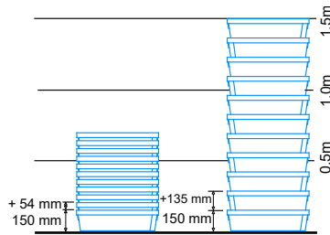
Ref. 990__ (ext.) 600x400x150mm (int.) 490x332x145mm 25L
