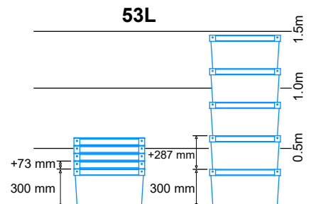
Ref. 130_ (ext.) 600x400x300mm (int.) 530x340x272mm
