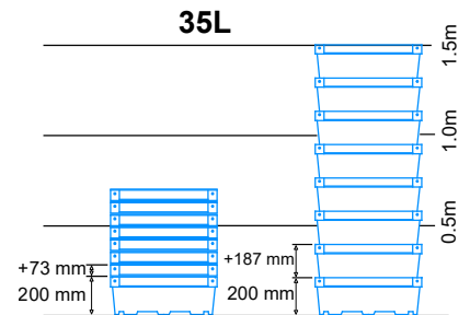
Ref. 120_ (ext.) 600x400x200mm (int.) 530x340x172mm
